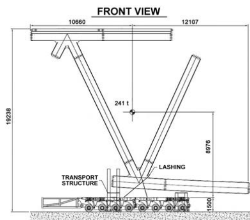
Figure 34. Drawing and photograph of self-propelled platforms.
