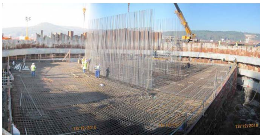
Figure 10. Reinforcement for P5 pile cap (30 m × 24.5 m × 4.5 m).
